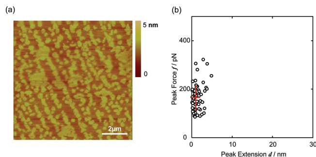
Figure 5. AFM contact-mode height image with untreated tips (a) and the scattering plot for the peak force and peak extension between a lysenin-conjugated tip and a binary-mixture bilayer of 1:1 PSM + DOPC on mica (b). The loading force and loading speed for force measurement were fixed at 300 pN and 500 nm s -1 , respectively. This plot is composed of 61 points, and the average values are \bar{f} = 172 \pm 54 pN and \bar{d} = 1.5 \pm 1.1 nm, indicated by the cross.
