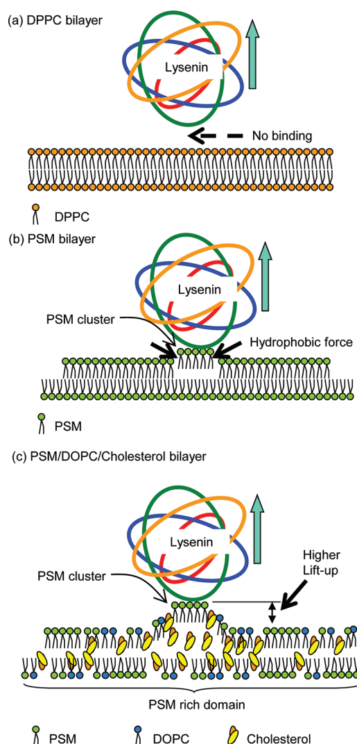
Figure 8. Schematic illustration for PSM cluster sliding motion upon attachment to lysenin and lifting up motion: (a) pure DPPC bilayer, (b) pure PSM bilayer, (c) PSM + DOPC + cholesterol bilayer.
