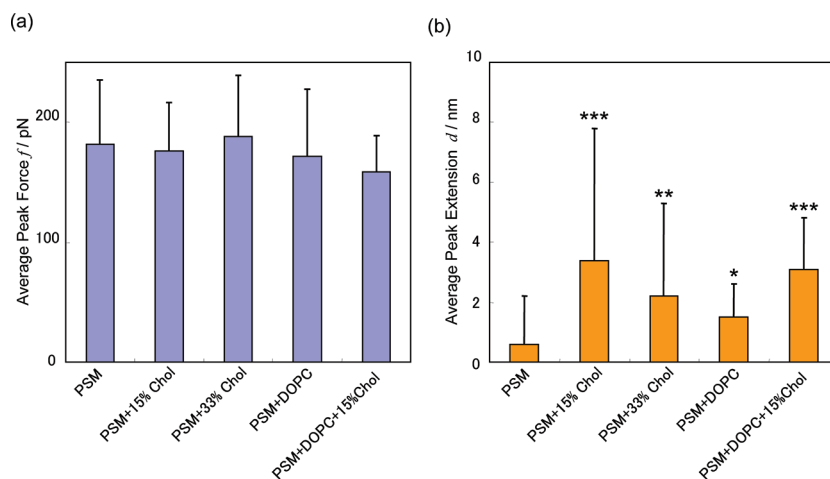
Figure 7. Summary for the average values of (a) peak force and (b) peak extension for the PSM-containing bilayers in Figures 4–6. In (b), the matching probability P with the pure PSM bilayer, calculated by Student's t test, are indicated as follows: *, P < 0.01; **, P < 0.002; ***, P < 0.001.
