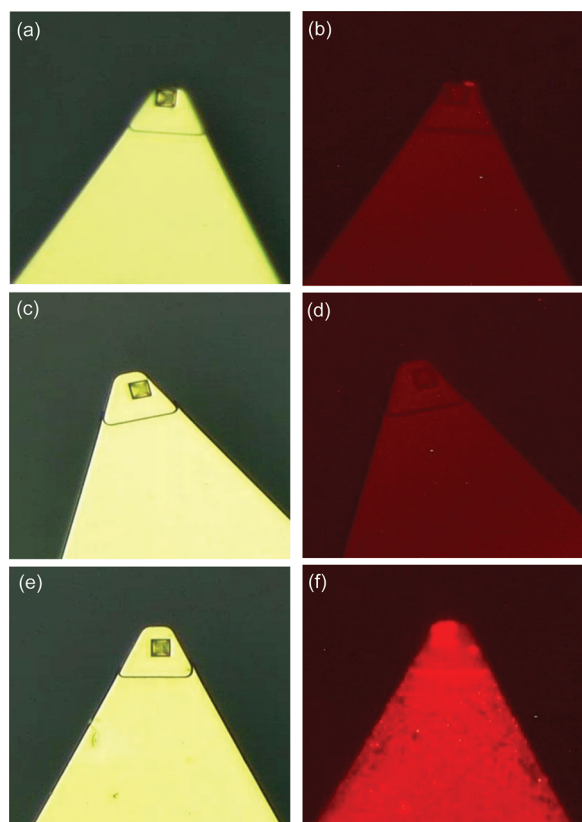
Figure 1. Optical microscopic images of an AFM tip/cantilever assembly before and after conjugation of lysenin to the surface. (a, b) The AFM tip was treated with 3-(mercaptopropyl)trimethoxysilane. (c, d) The tip in (a, b) was further treated with bifunctional cross-linker, N -succinimidyl pyridyldithiopropionate (SPDP). (e, f) The tip in (c, d) was further treated in the solution of RFP-lysenin. (a, c, e) Bright field image. (b, d, f) Fluorescence image.
