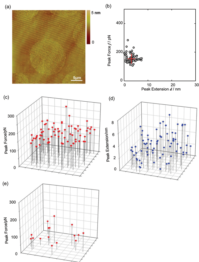
Figure 6. AFM contact-mode height image (a) and the distribution of the peak force/peak extension between lysenin and the ternary mixed PSM/DOPC/cholesterol (42.5:42.5:15) bilayer. (b) The scattering plot for the peak force and peak extension. 71 points, \bar{f} = 157 \pm 34 pN and \bar{d} = 3.08 \pm 1.78 nm. The loading force and loading speed for force measurement were fixed at 300 pN and 500 nm s -1 , respectively. (c) Two-dimensional distribution of binding force for the SM-rich area (2 μm × 2 μm divided into 81 (9 × 9) points) were selected for force recording. (d) Two-dimensional distribution of peak extension for the same area. (e) Two-dimensional distribution of binding force recorded in SM-poor area. The force mapping was operated in a 2 μm × 2 μm square area, divided into 72 (8 × 9) points. Initial loading force = 300 pN. The points where the peak force was less than 20 pN were not plotted.
