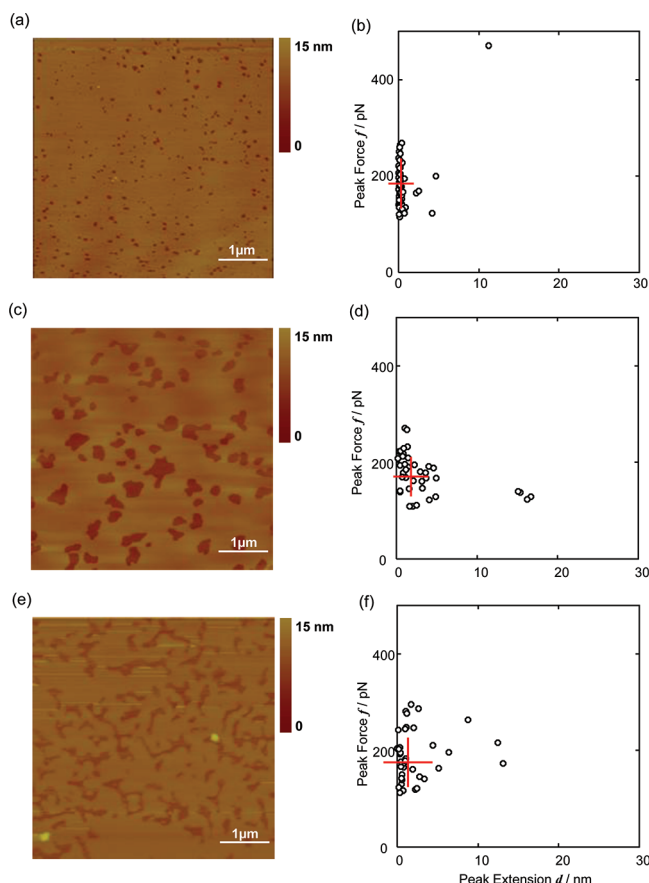
Figure 4. AFM contact-mode height image with untreated tips and the scattering plots for the peak force f and peak extension d between lysenin-conjugated tips and pure PSM or PSM/cholesterol bilayer on mica. The loading force and loading speed for force measurement were fixed at 300 pN and 500 nm s -1 , respectively. (a, b) For pure PSM. The scattering plot contains 63 points. The averages, \bar{f} = 182 \pm 53 pN and \bar{d} = 0.6 \pm 1.6 nm, are indicated by a cross in the plane. (c, d) 85:15 PSM + cholesterol, 39 points, \bar{f} = 176 \pm 41 pN and \bar{d} = 3.4 \pm 4.4 nm. (e, f) 67:33 PSM + cholesterol, 39 points, \bar{f} = 188 \pm 51 pN and \bar{d} = 2.2 \pm 3.1 nm.
