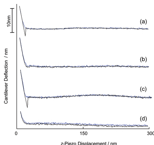
Figure 2. Typical raw force curves, represented as z -piezo displacement/nm versus cantilever deflection/nm, of the tip-conjugated lysenin to different membranes. Blue lines indicate approaching curves whereas black lines show retraction curves. The force constants of cantilevers used were 50 pN nm -1 in average, and the scanning speed for z -piezo displacement was 500 nm s -1 both for approaching and retracting (loading rate in approach = 2500 pN s -1 ). (a) A typical force curve obtained with lysenin-attached tip on a bilayer of N -palmitoyl- D -erythro-sphingosylphosphorylcholine (PSM). Loading force = 300 pN. (b) A force curve on a bilayer of 1,2-dipalmitoyl- sn -glycero-3-phosphocholine (DPPC). Loading force = 300 pN. (c) A force curve with lysenin-attached tip on a PSM/1,2-dioleoyl- sn -glycero-3-phosphocholine (DOPC) (1:1) bilayer. Loading force = 400 pN. (d) A force curve with lysenin-attached tip on a bilayer of PSM/DPPC (1:1). Loading force = 200 pN.
