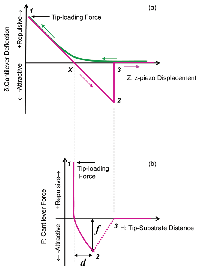
Figure 3. Schematic representation of an AFM force–distance cycle with lysenin-attached tip on sphingomyelin (SM)-containing membrane. Frame (a) schematizes the raw force curves, indicating the cantilever deflection ( \delta/\text{nm} ) as a function of z -piezo displacement ( Z/\text{nm} ). The tip was moved toward the membrane surface (on green line, toward point 1) and subsequently retracted (pink line, toward point 2) with the in-plane tip position fixed. During tip approach, lysenin binds to SM, leading to a force signal with a distinct shape (point 1 to point 2) while the tip is retracted. The force increases until the dissociation occurs (from point 1 to point 2). The raw force curves were numerically converted by eq 1 in the text into the force ( F/\text{pN} ) as a function of the tip–substrate distance ( H/\text{nm} ), shown in frame (b). When the dissociation occurs (point 2), the cantilever returns to the neutral position and the tip travels back to point 3 by the distance of deflection. The negative peak at point 2 provides two characteristic parameters, that is, the peak extension ( d/\text{nm} ) and the peak force ( f/\text{pN} ). The peak extension is given as the distance of the negative peak position from the zero-cross point ( X ) of the F – H curve. The peak force is the depth of negative peak.
